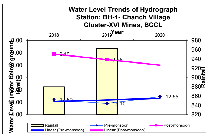
Figure No-11: Groundwater Level Hydrographs of the Borehole.
